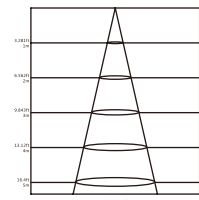
Illuminance Characteristics
