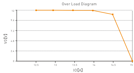
LM-150-12-G1T2
