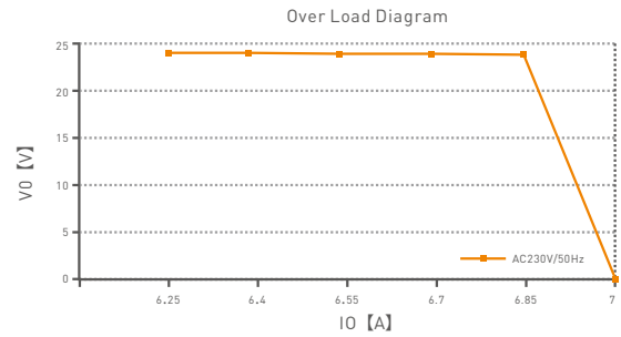
LM-150-24-G1T2
