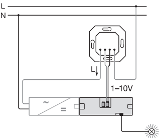
1-10 V dimmer connection diagram
