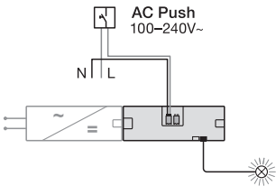
Mains voltage push button connection diagram
