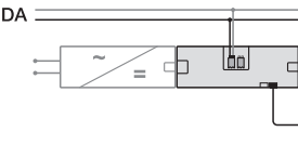
DALI-2™ connection diagram
