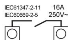
connection plan RM16 IS HS
