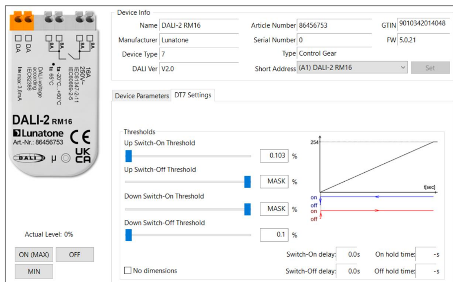
Figure 1 DALI Cockpit tab: DT7 settings
