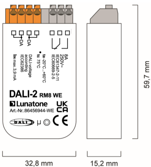
geometry RM8 WE
