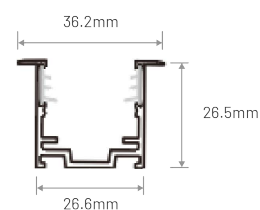
F2219 Flange Serrated Aluminum Profile
