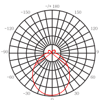
Candle power distribution
