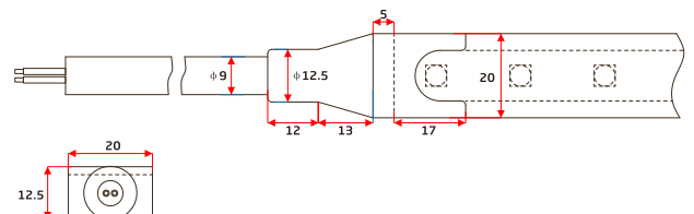
Injection-moulded Front Connector(top end)
