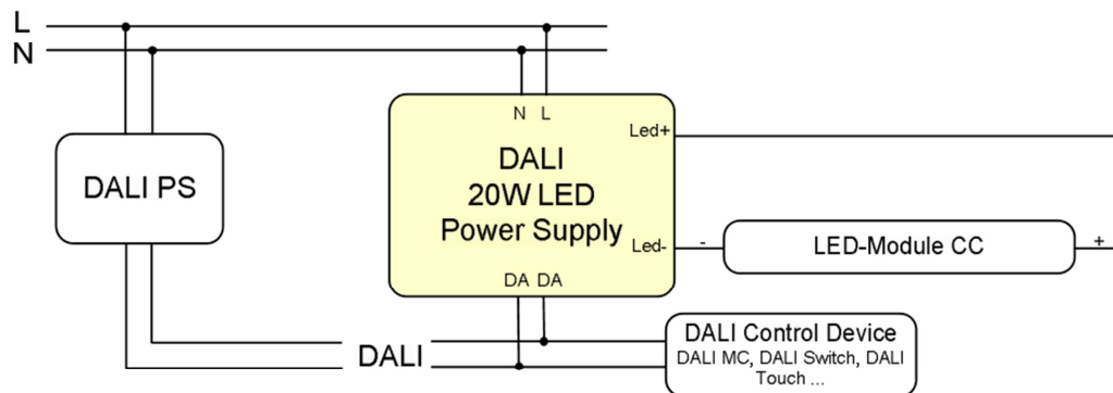
typical installation
